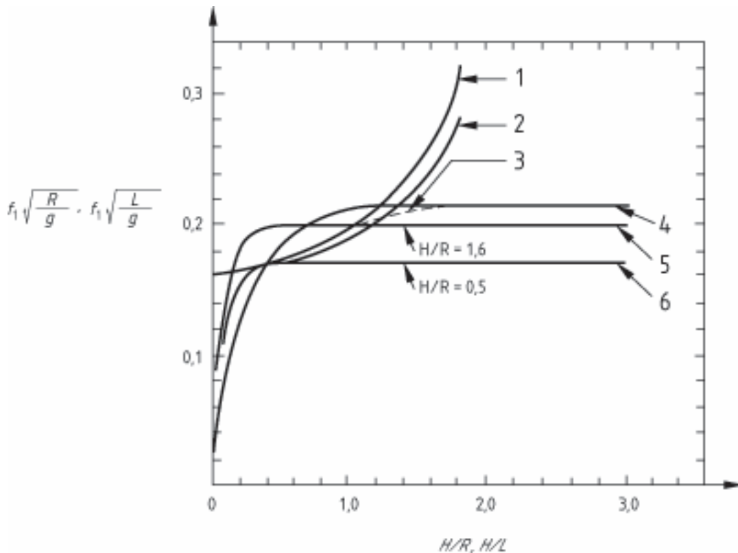
Figure A.10 — Dimensionless first convective mode frequency for rigid tanks of various shapes [8]
