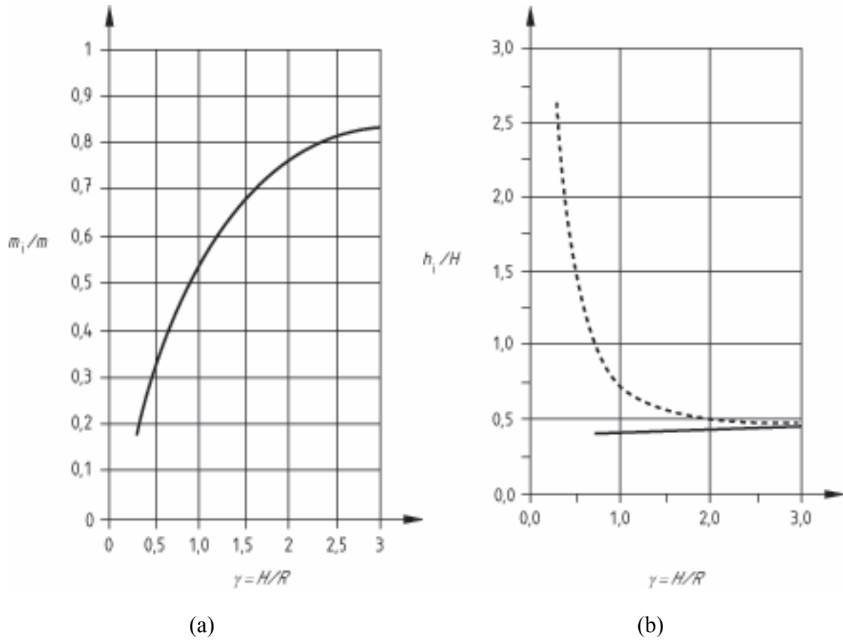
Figure A.2 — Ratios m_i/m , h_i/H and h'_i/H as functions of the tank slenderness (see also Table A.2, columns 4, 6 and 8)
