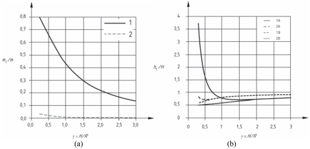
Figure A.4 — a) First two sloshing modal masses and b) corresponding heights h_{c1} , h_{c2} , h'_{c1} and h'_{c2} as functions of \gamma (see also Table A.2, columns 5, 7 and 9)
